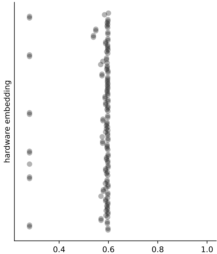
horizon = 1
